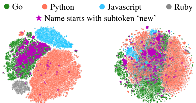
Figure 3: t-SNE visualization of the representation learned by MetaTPTrans- \alpha (left) and TPTrans (right).
