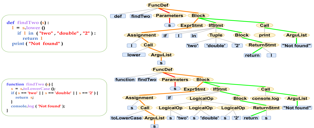
Figure 1: The same code snippet and its associated AST in Python (top) and JavaScript (bottom).
