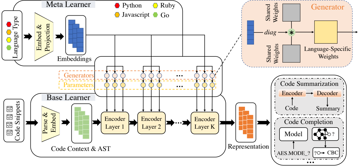
Figure 2: Architecture of MetaTPTrans.
